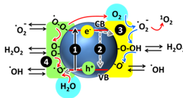
Figure 1. Reactive oxygen species generated in the photocatalytic reduction and oxidation steps of oxygen and water. Absorption of light (1) causes the transition of electrons to the conduction band and the formation of holes in the valence band. Part of the produced charges undergo recombination (2), whereas others migrate to the surface where trapped electrons (3) participate in the reductive steps (blue arrows) and trapped holes (4) in the oxidative processes.
