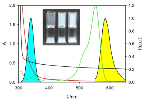
Figure 5. Absorption spectrum of hydrogel 1 (H) (black line) of the \text{TiO}_2 NPs (0.2 mg/mL, red line) and RhB ( \times 20 , 1 \mu\text{M} , green line). Fluorescence spectrum of RhB (filled yellow) and spectrum of the irradiation source (filled cyan). Inset: photographs of samples of hydrogels 1 (H), 2 (H-T), and 3 (H-TG) (from left to right, respectively) prepared with gelator Fmoc-L-Tyr-D-Oxd-OH in 0.5% concentration.
